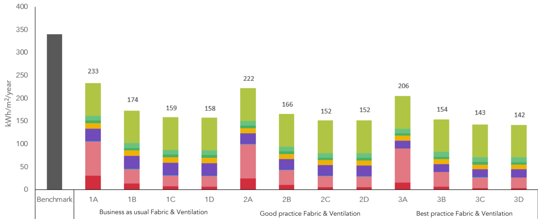
Figure 7.8 - Predictive energy modelling results: bar chart showing the detailed breakdown of energy use intensity (EUI) for each case
