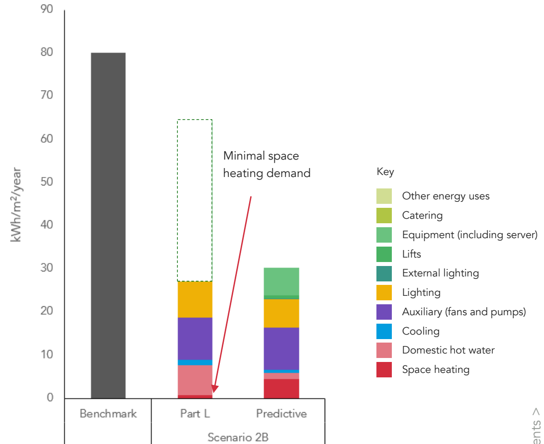
Figure 8.7 – Comparison between the results of the Part L energy model and the Predictive energy model, per separable energy use, for a typical 'good practice' scenario with a heat pump
