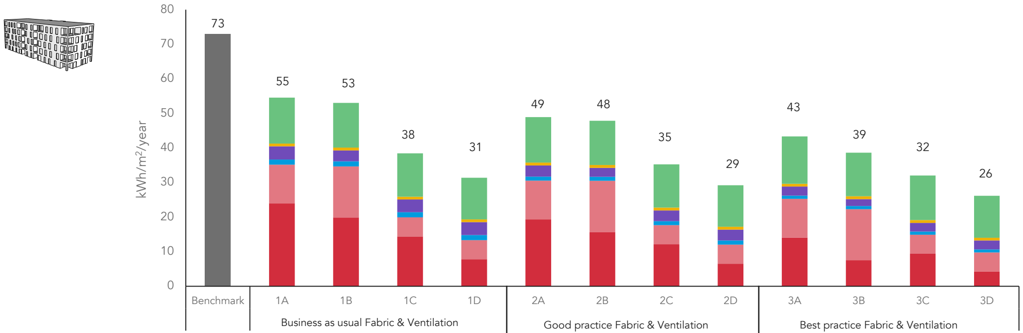
Figure 7.3 - Predictive energy modelling results: bar chart showing the detailed breakdown of energy use intensity (EUI) for each case
