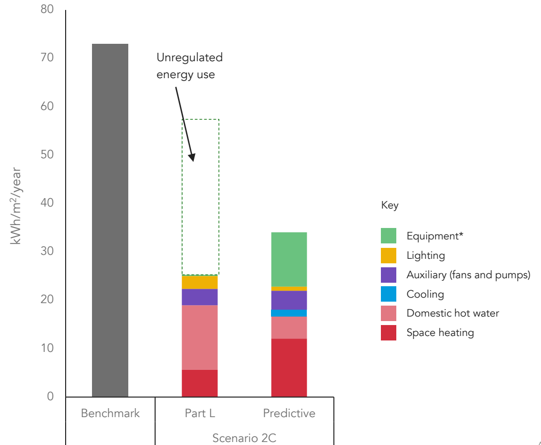
Figure 8.1 – Comparison between the results of the Part L energy model and the Predictive energy model, per separable energy use, for a typical 'good practice' scenario with a heat pump
