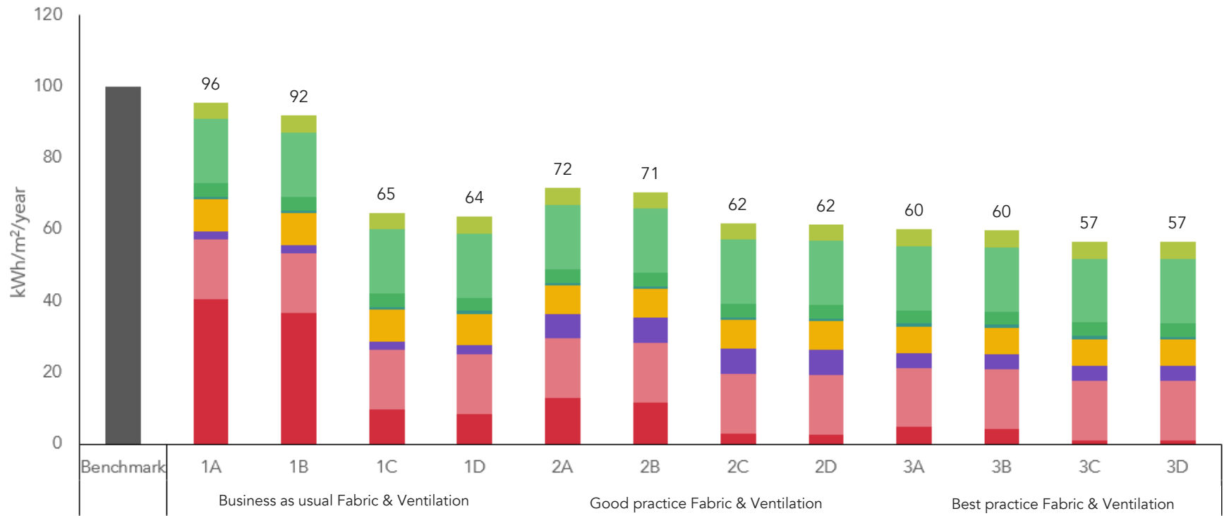
Figure 7.6 - Predictive energy modelling results: bar chart showing the detailed breakdown of energy use intensity (EUI) for each case
