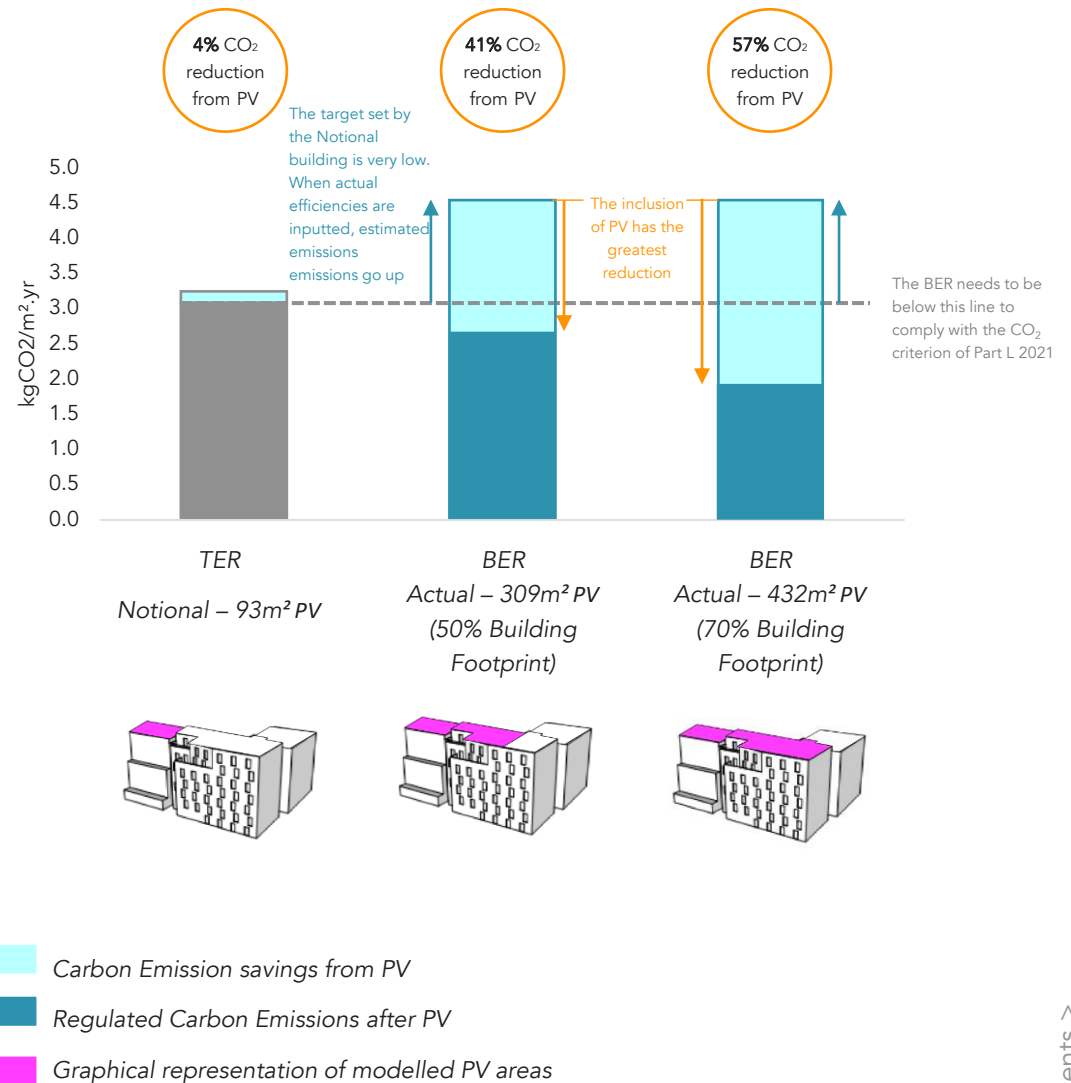
Figure 6.6 - The above chart shows that regulated carbon emissions forming the Part L 2021 limit which new buildings have to comply with is very challenging: the emissions are very low. In the actual building, even when good/best practice specifications are assumed, the building's emissions are estimated to be much higher, relying on PVs to comply. The example used above is the office building.
