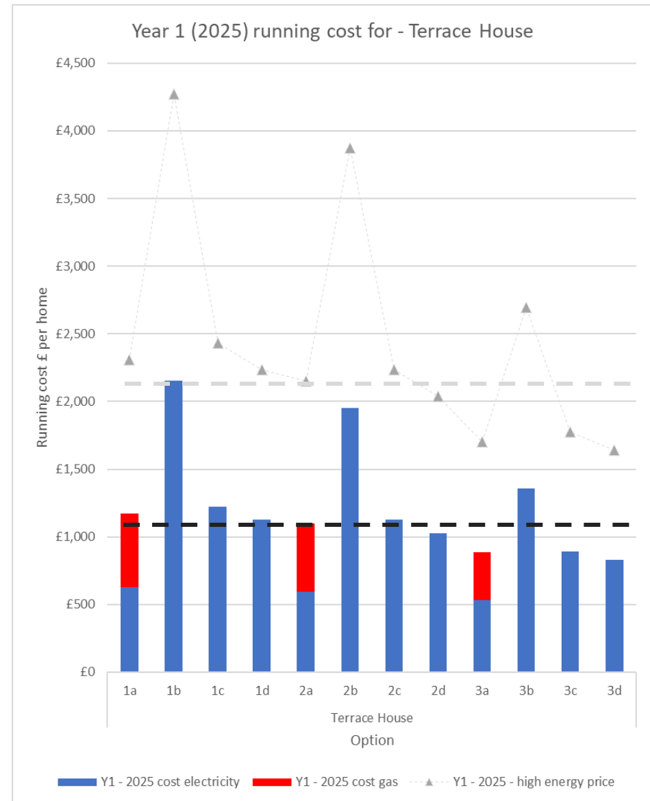
Figure 9.4 – Estimated year 1 energy costs for each case
