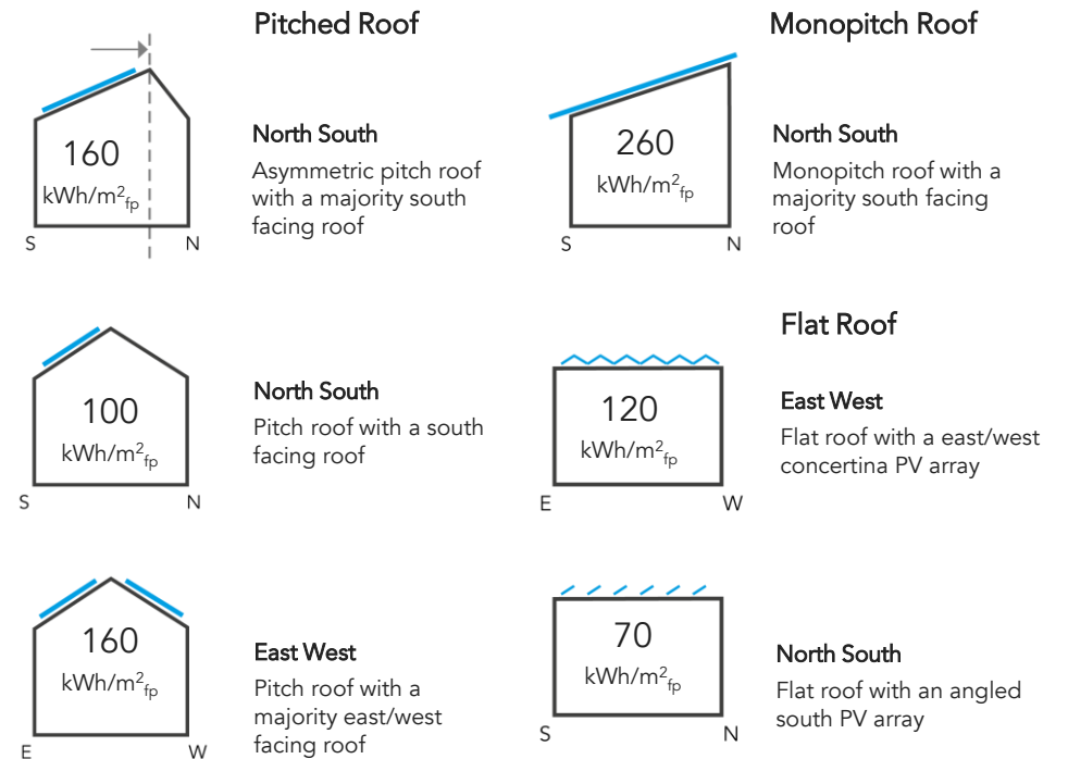
Figure 11.13 - Roof design can be optimised to maximise energy output from photovoltaics. A useful indicator of this is expressed in kWh generated per \text{m}^2 of building footprint ( \text{kWh/m}^2_{\text{fp}} )
