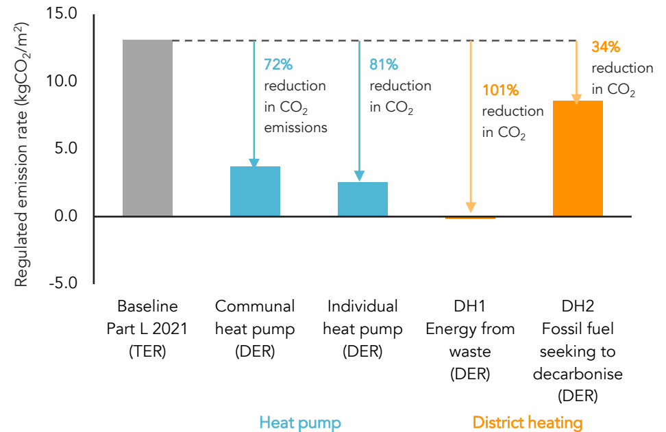
Figure 6.9 - Analysis of district heating and comparison with heat pump scenario
