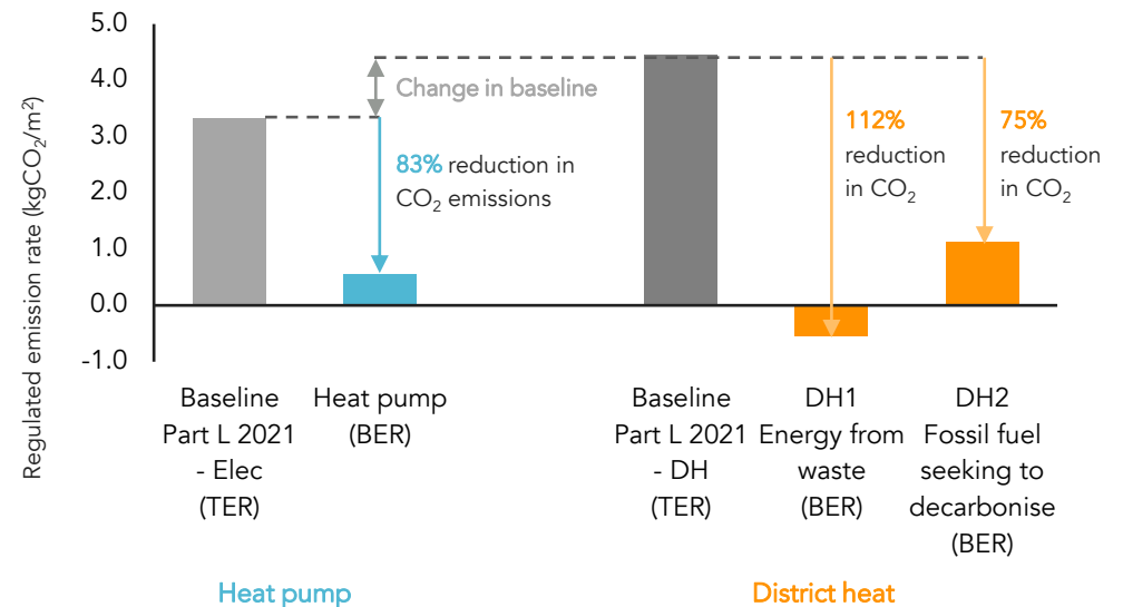
Figure 6.7 - Analysis of district heating and comparison with heat pump scenario: comparison of results from a heat pump (ground Source heat pump or ambient loop) and district heating scenarios.
