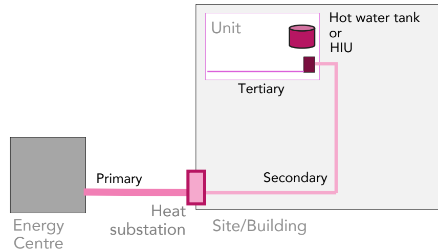
Categories of distribution and standing losses on a heat network
