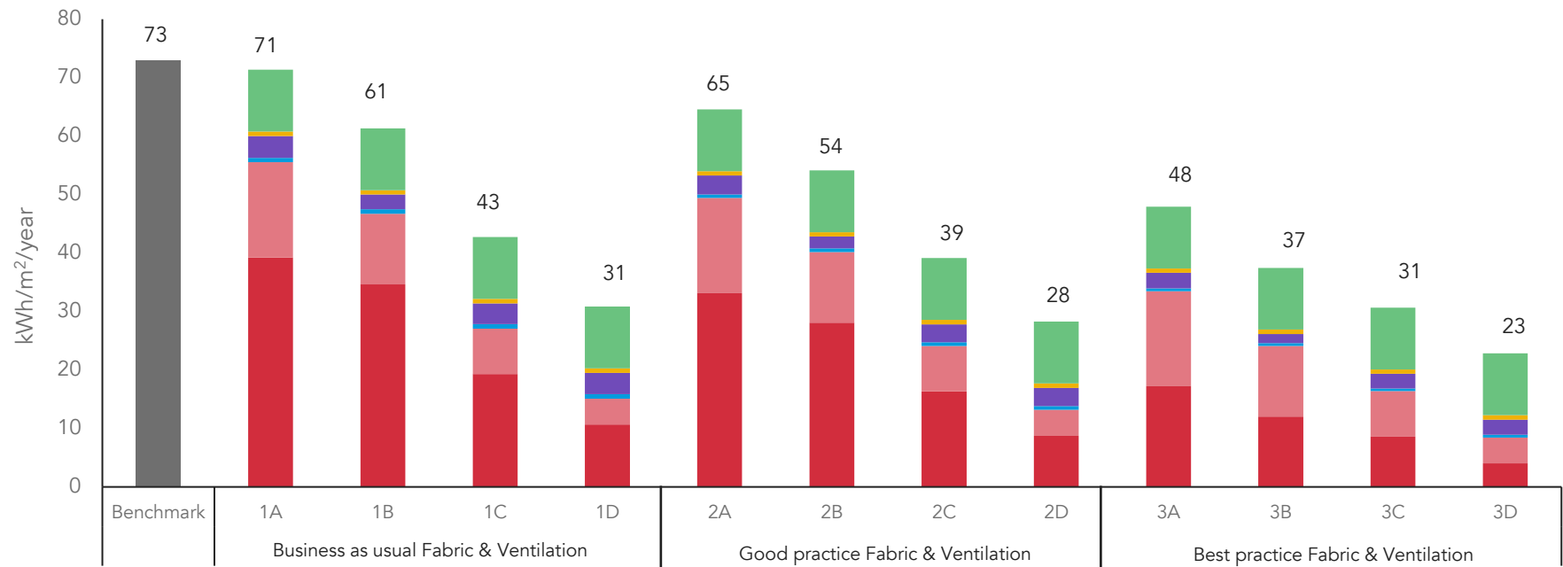
Figure 7.2 - Predictive energy modelling results: bar chart showing the detailed breakdown of energy use intensity (EUI) for each case
