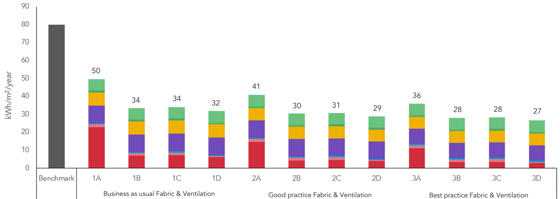
Figure 7.7 - Predictive energy modelling results: bar chart showing the detailed breakdown of energy use intensity (EUI) for each case
