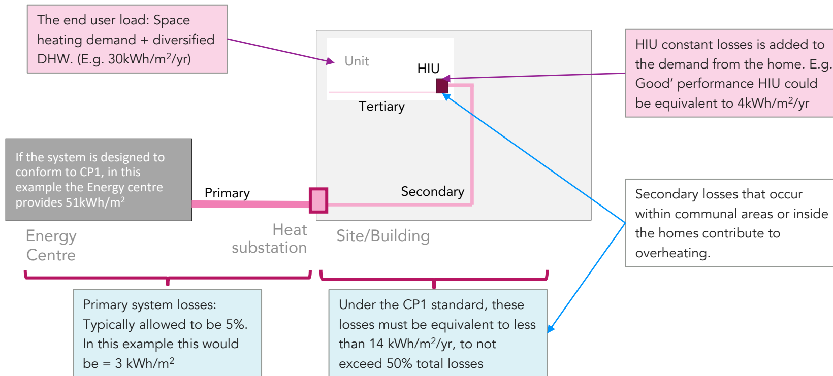
Figure 10.2 - Example of distribution losses on a heat network
