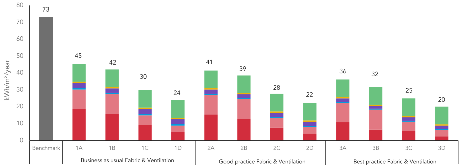
Figure 7.4 - Predictive energy modelling results: bar chart showing the detailed breakdown of energy use intensity (EUI) for each case
