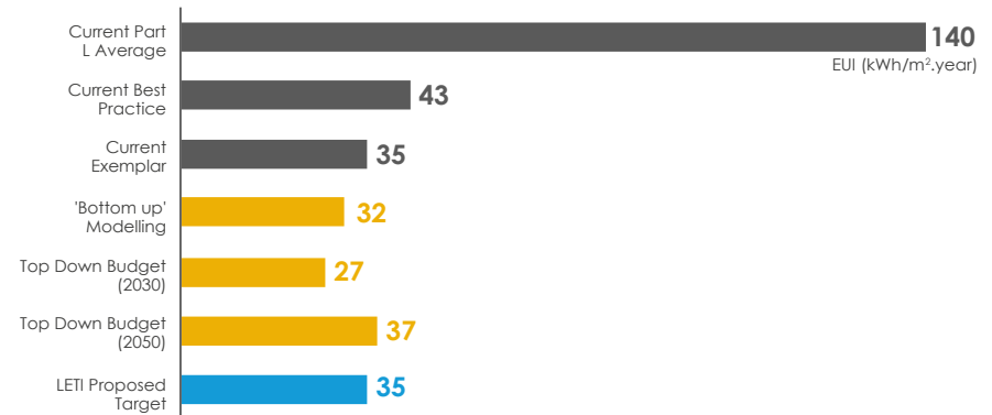
Figure 11.6 - LETI domestic top-down analysis taken from LETI Climate Emergency Design Guide
