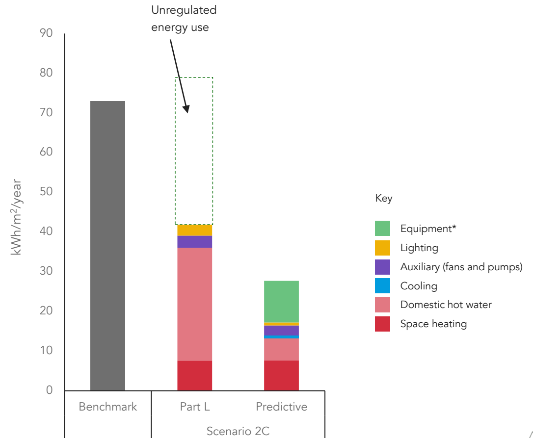
Figure 8.4 – Comparison between the results of the Part L energy model and the Predictive energy model, per separable energy use, for a typical 'good practice' scenario with a heat pump
