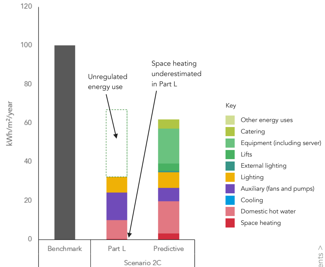
Figure 8.6 – Comparison between the results of the Part L energy model and the Predictive energy model, per separable energy use, for a typical 'good practice' scenario with a heat pump
