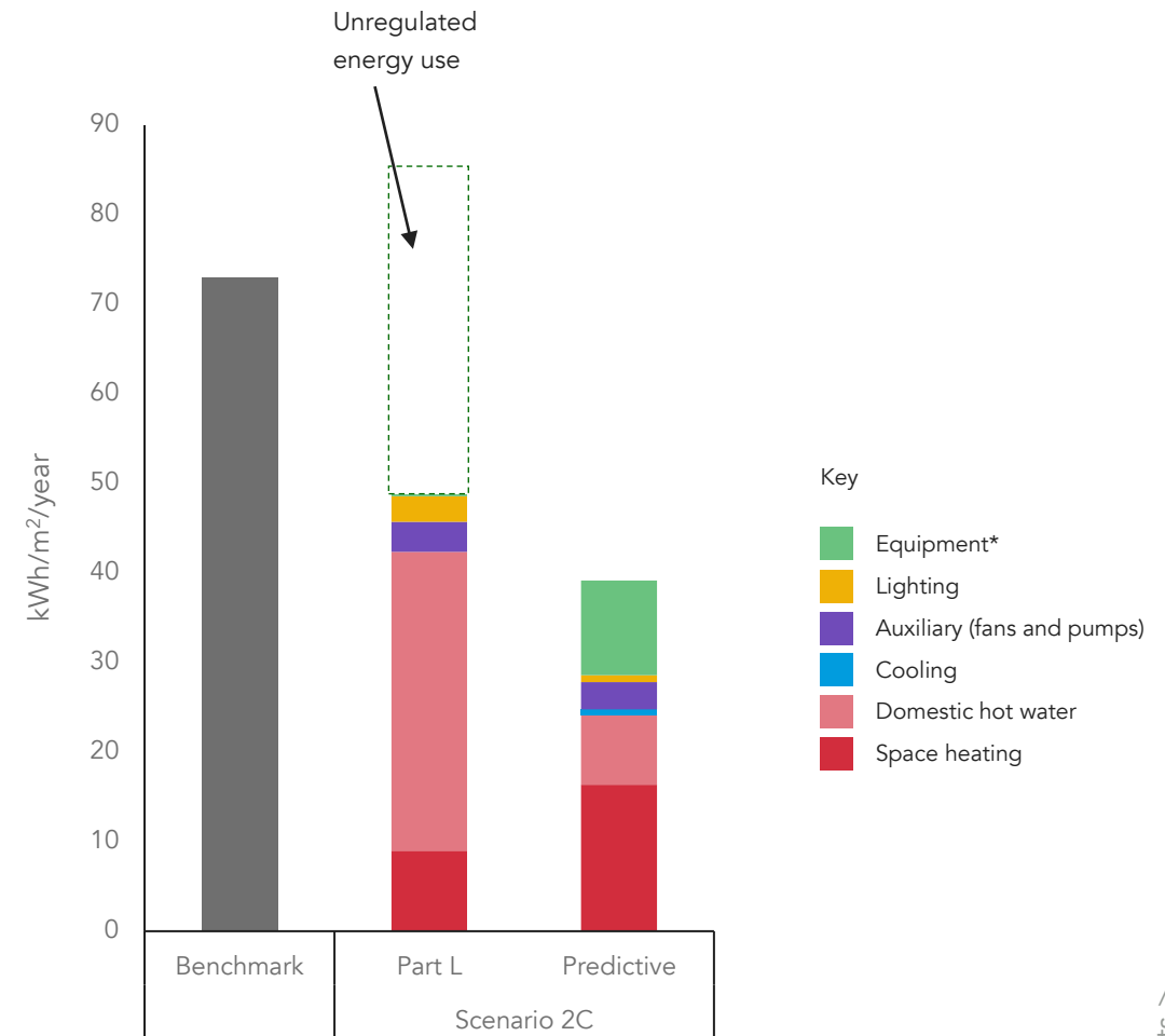
Figure 8.2 – Comparison between the results of the Part L energy model and the Predictive energy model, per separable energy use, for a typical 'good practice' scenario with a heat pump
