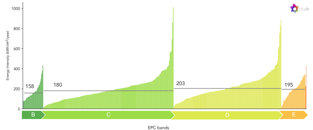
Figure 11.14 - EPC data compared with measured energy consumption of 420 homes. There is little correlation and only marginal improvement on average energy consumption per EPC rating which demonstrates the existence of a performance gap between intended and actual energy performance.
