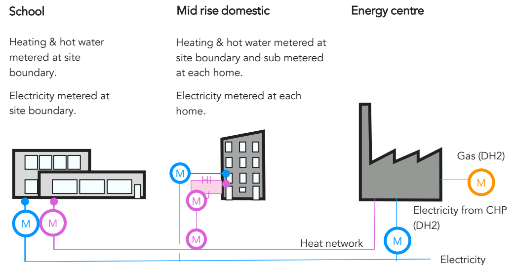
Figure 7.10 - The image above illustrates the metering strategy typically employed when delivering heat from a DH network and the metering strategy for electrical consumption. It should be recognised that where Combined Heat and Power generation is adopted, there will be a rebate due to the generation of electricity.
