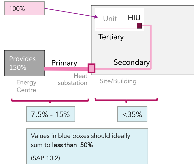
Breakdown of distribution losses to comply with the CIBSE CP1 design requirements.
