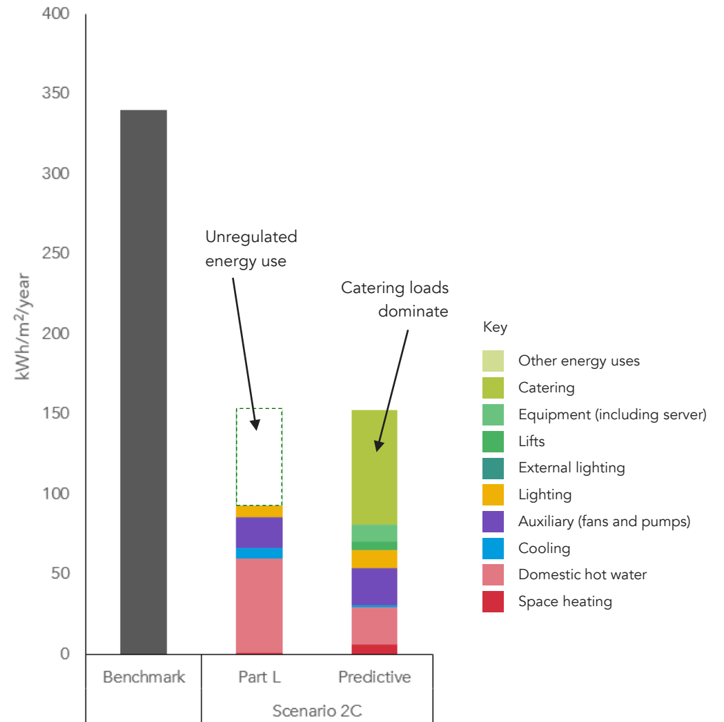
Figure 8.8 – Comparison between the results of the Part L energy model and the Predictive energy model, per separable energy use, for a typical 'good practice' scenario with a heat pump
