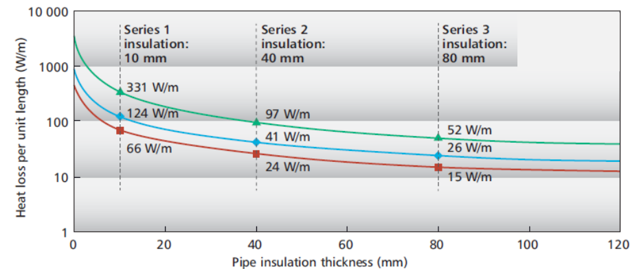
Figure 30 Indicative heat losses from insulated pipes and relative performance of Series 1–3 insulation (for a pair of flow and return pipes at fixed ambient and fluid temperatures) (source: GLA, 2014)
