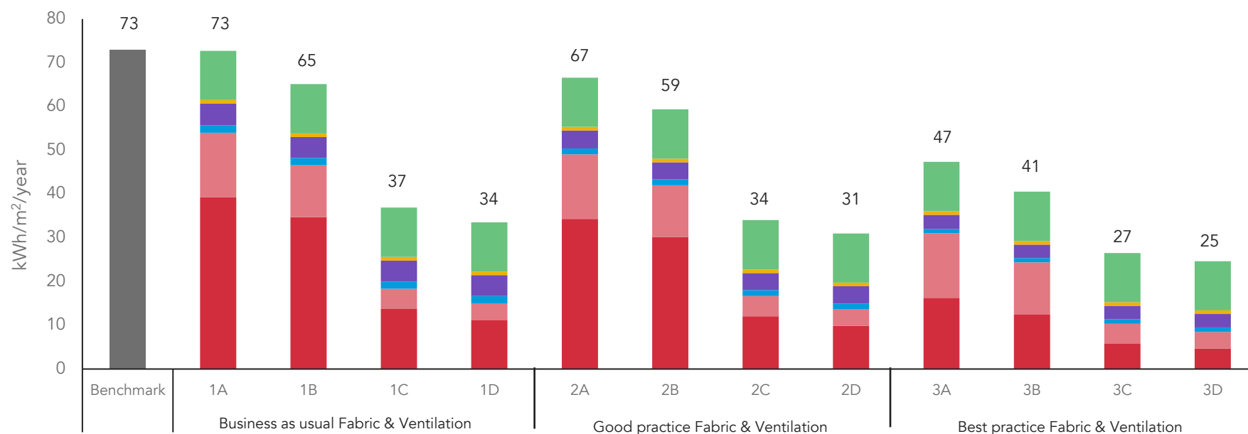
Figure 7.1 - Predictive energy modelling results: bar chart showing the detailed breakdown of energy use intensity (EUI) for each case
