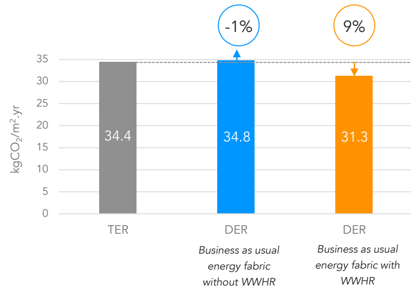
Figure 6.5 - The chart above shows the impact of WWHR on the GLA ‘Be Lean’ case in a mid-rise apartment building. A significantly greater reduction in CO 2 emissions is achieved when WWHR is included in the proposed building specification.
