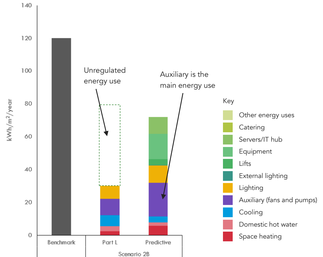
Figure 8.5 – Comparison between the results of the Part L energy model and the Predictive energy model, per separable energy use, for a typical 'good practice' scenario with a heat pump
