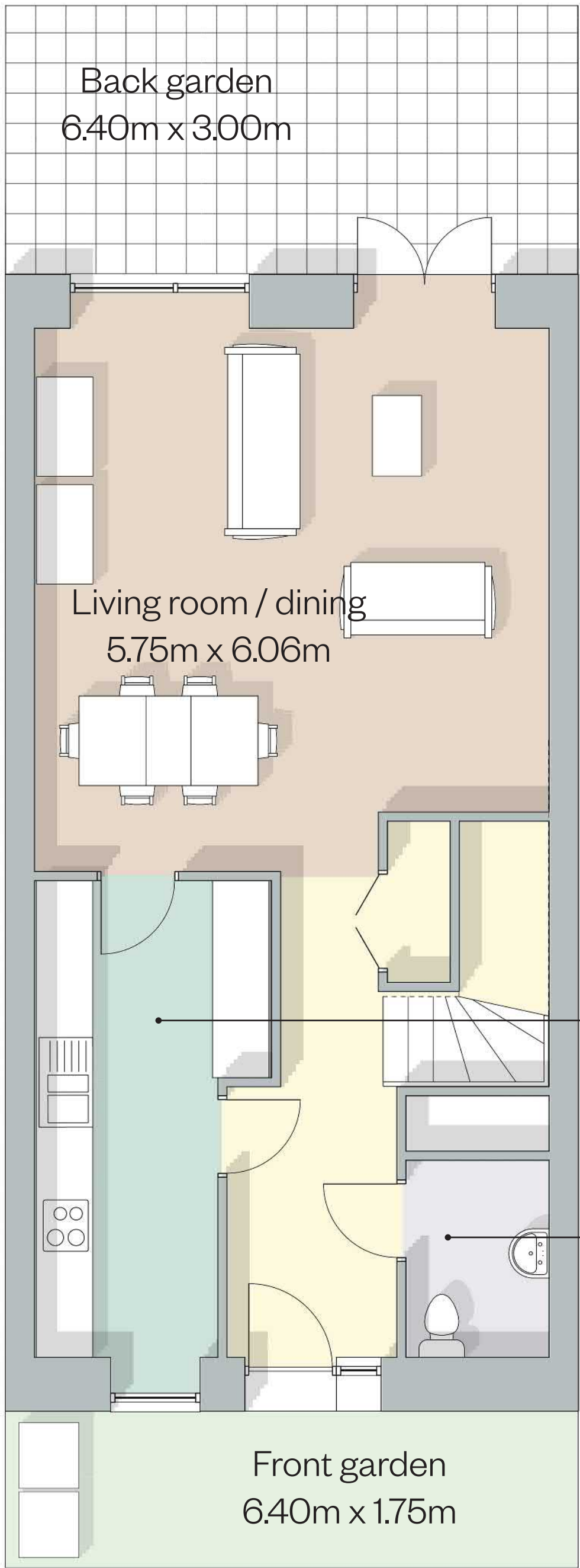
Floor Plan 1: 50
